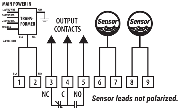
FIGURE 1 – WIRING DIAGRAM (RS-092-MK2 SHOWN)
